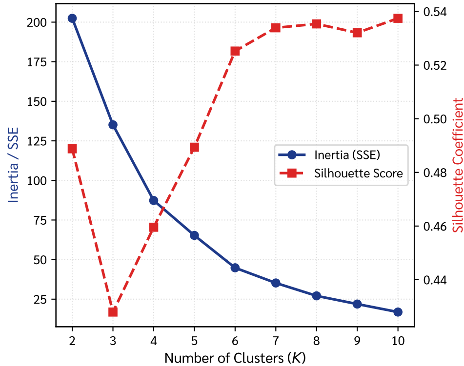
(b) Metric Curves ( K = 2 \dots 10 )
