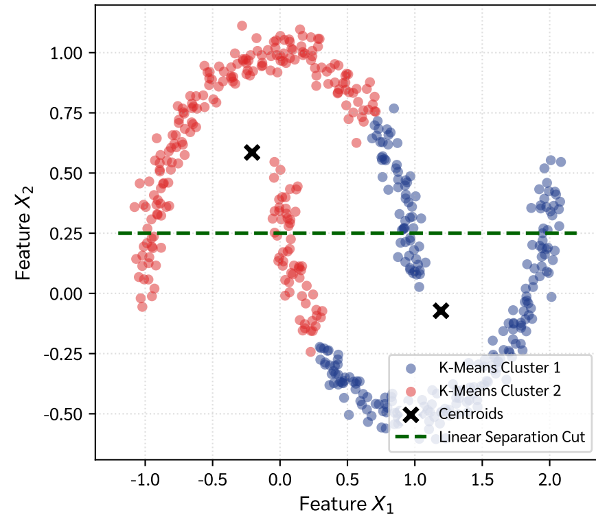
(c) K-Means Failure ( K = 2 , Manifold Cut)
